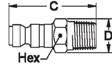
Figure 4 (Tru-Flate)
